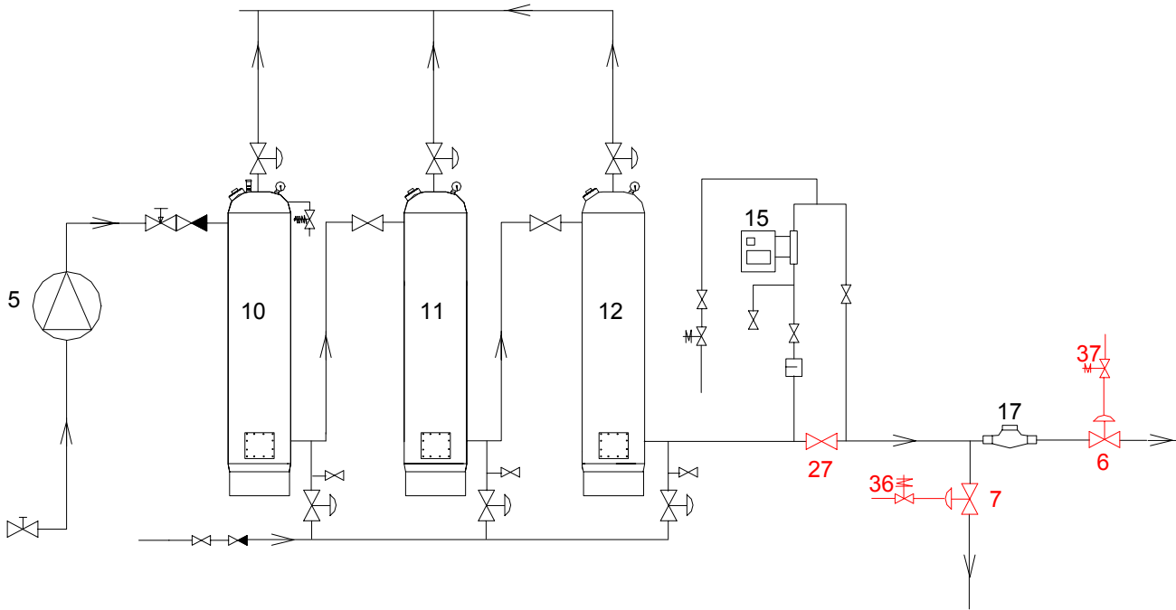
Ball valve on adjustment valve #27
